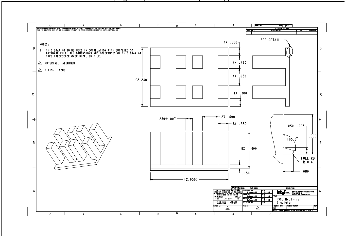
Figure 4. Schematic of heat sink simulator for mechanical shock and vibration tests.
